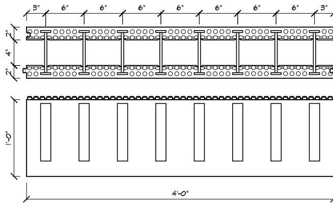
2-4-2 STANDARD (PLAN/SIDE)
