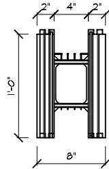
END VIEW 2-4-2
