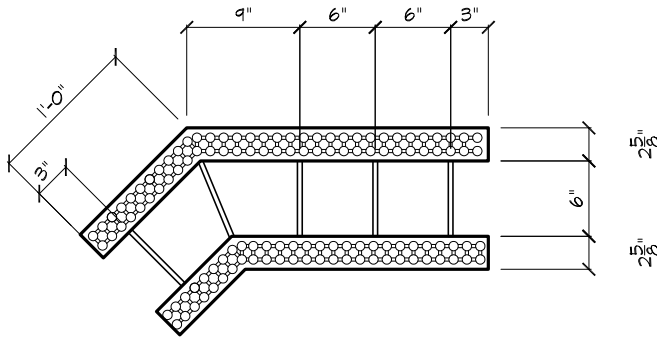
6" 45° CORNER BLOCK (LEFT/RIGHT)
