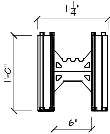
6" STANDARD BLOCK (END VIEW)
