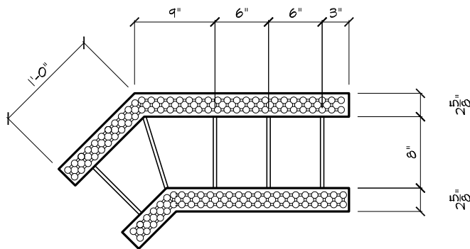
8" 45° CORNER BLOCK (LEFT/RIGHT)
