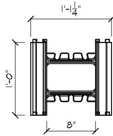
8" STANDARD BLOCK (END VIEW)
