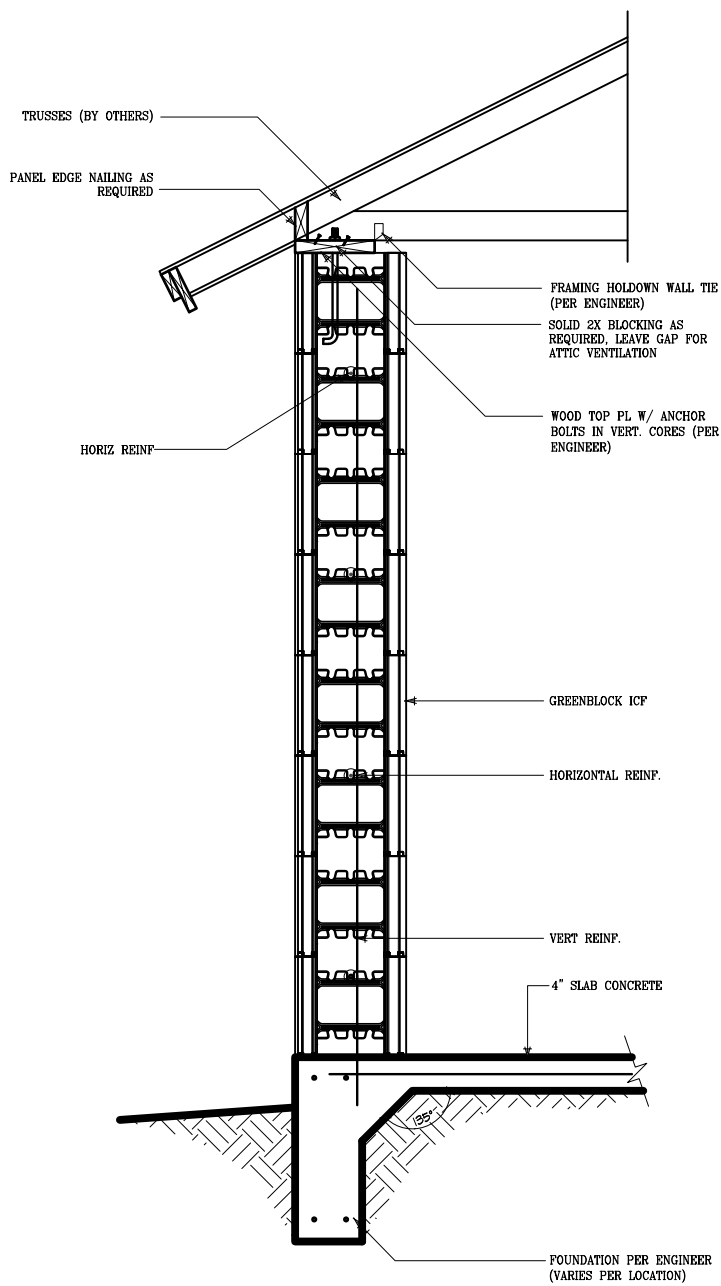
8" WALL TYPICAL CROSS SECTION
