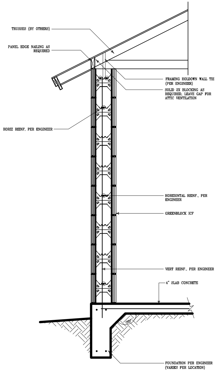
6" WALL TYPICAL CROSS SECTION
